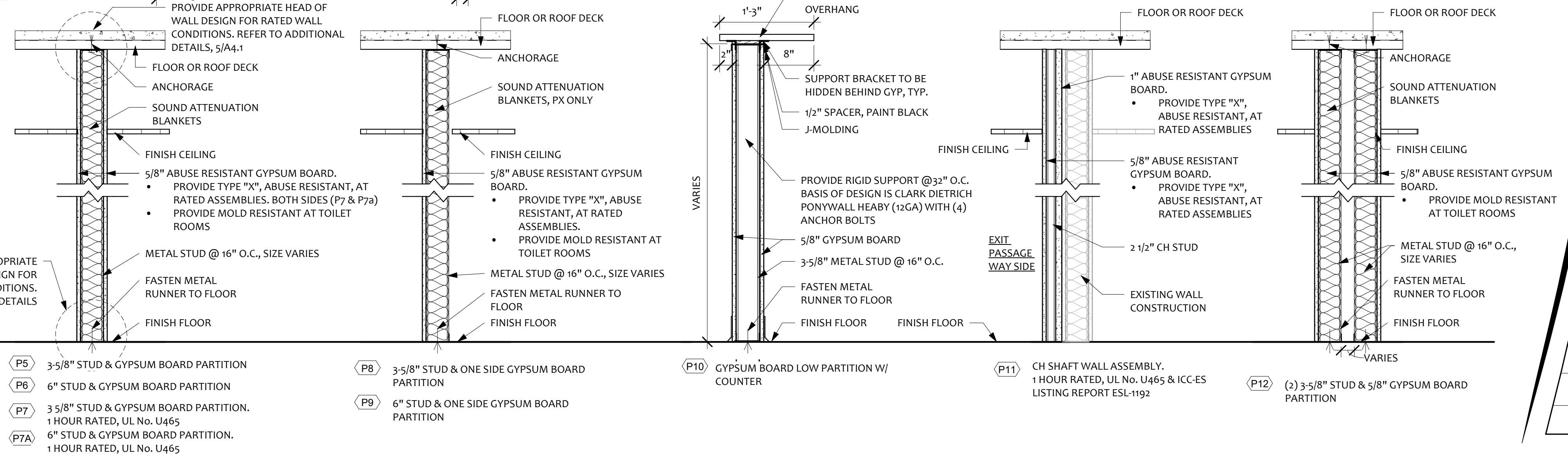
WALL PARTITIONS 1" = 1'-0"
